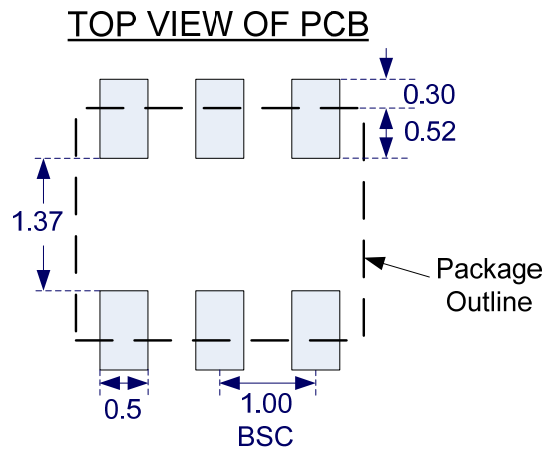
Fig. 15: LGA package land pattern (top view).
