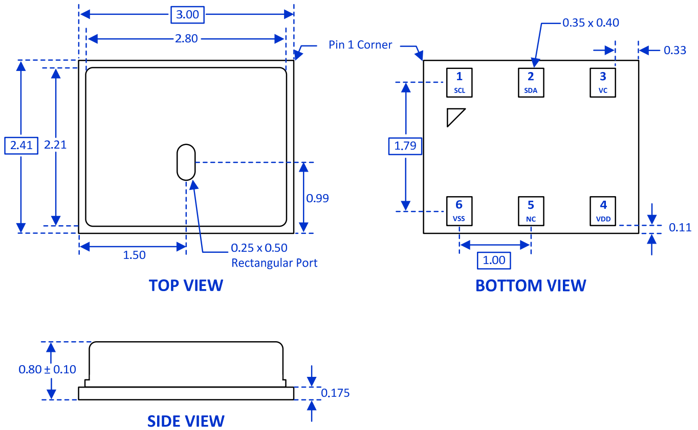
Fig. 14: LGA package drawing.
