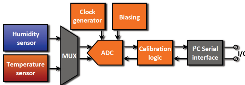
Fig. 4: MVH3200D series functional diagram.
