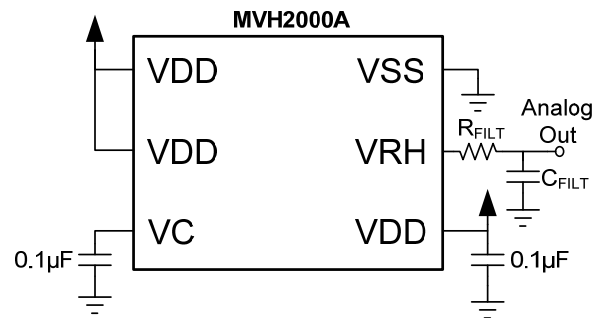
Fig. 3: Connection diagram.
