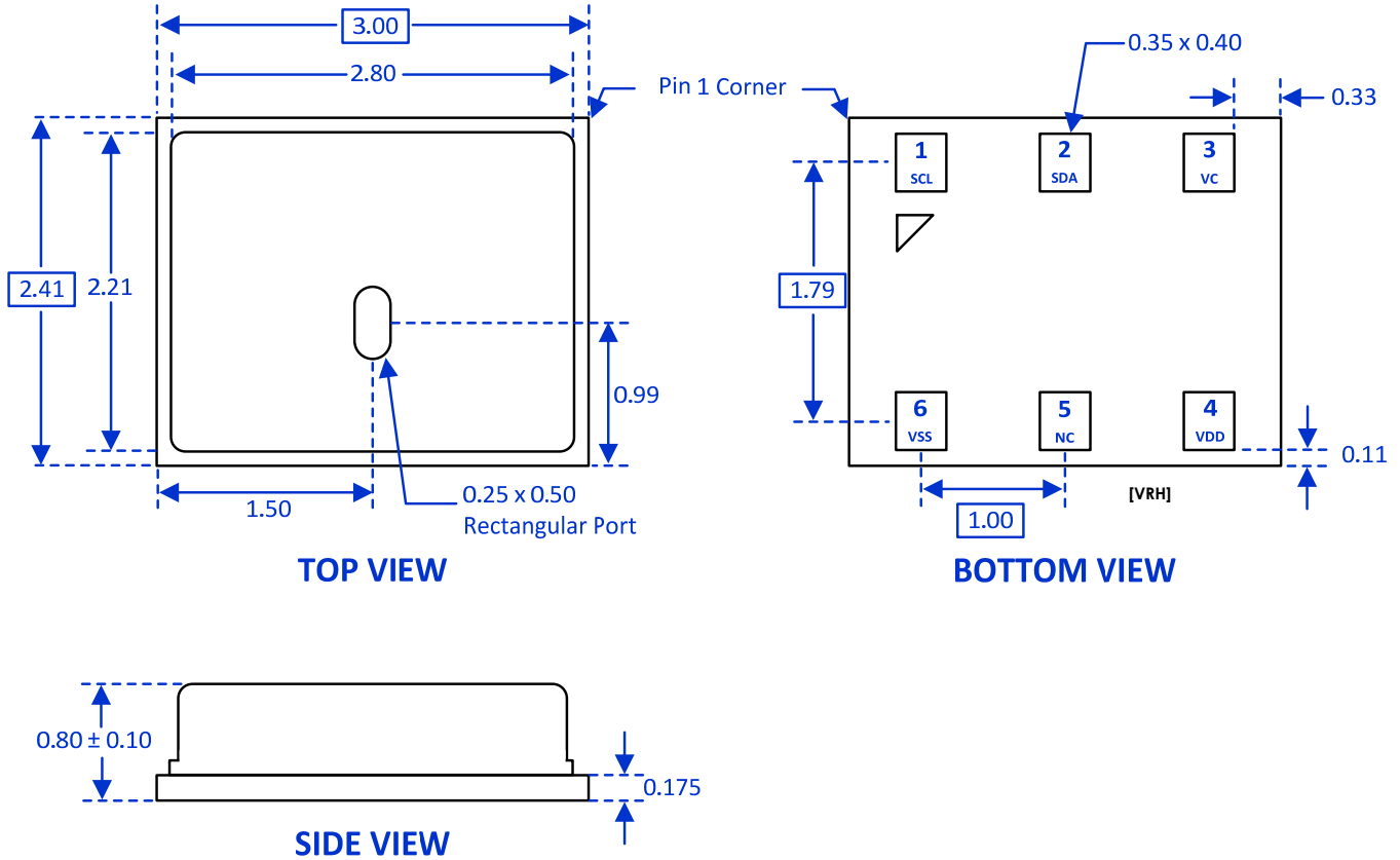
Fig. 8: LGA package drawing.
