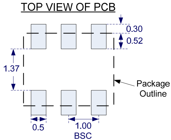
Fig. 9: LGA package land pattern (top view).
